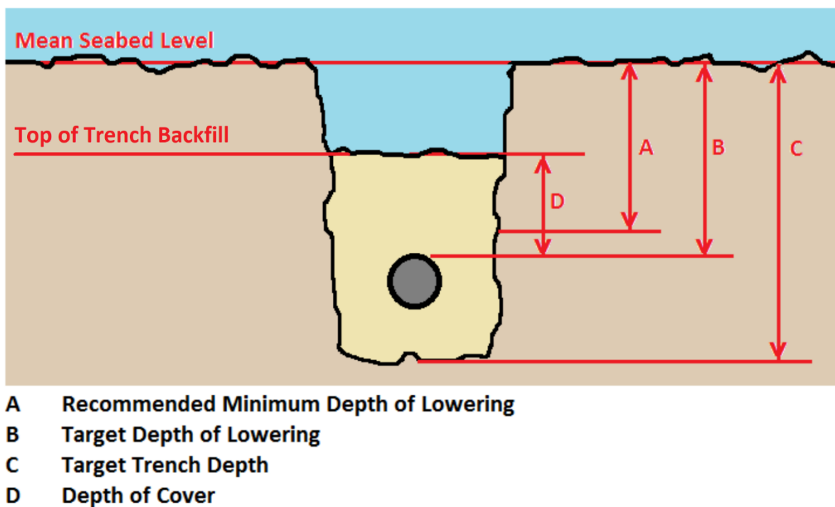
Figure 6: Definition of Trench Parameters and Abbreviations
